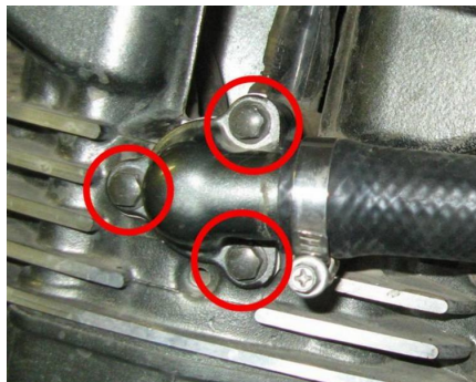
Figure 5. Original Thermostat Housing is restrained by 3 bolts.
